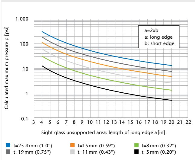
Rectangular sight glass at room temperature annealed BOROFLOAT® 33 (design strength 870 psi)
