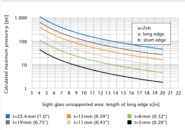
Rectangular sight glass at room temperature BOROFLOAT® 33 heat strengthened 2130 psi (design strength 3000 psi)
