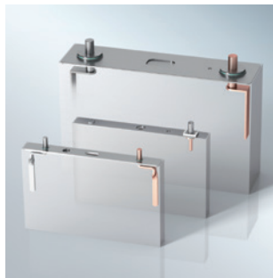
SCHOTT GTAS® – Lid systems for prismatic lithium ion batteries
