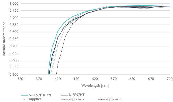
N-SF57HTultra, n_d = 1.84666 , v_d = 23.78
