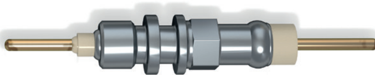
Glass seals maintain integrity
