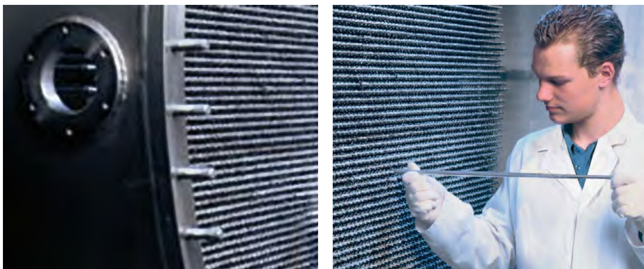
Three separate generators each with some 21,000 DURAN® glass tubes – 10,324 at each end – were installed in the world's largest ozone production system at VCP in Brazil. The outer and inner diameters of the special glass tubing required for the construction of the electrodes have an extremely narrow range of permissible variation.
