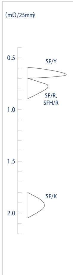
Internal resistance
